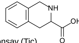
1,2,3,4-tetrahydroizokinolin-3-karbonsav (Tic)
