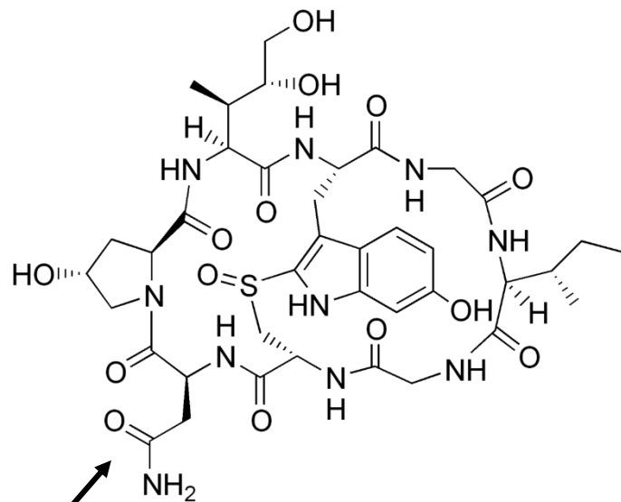
\alpha -anamitin
