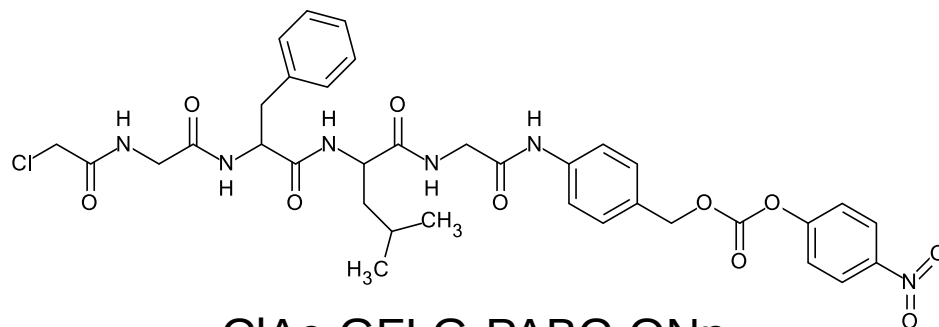
ClAc-GFLG-PABC-ONp
