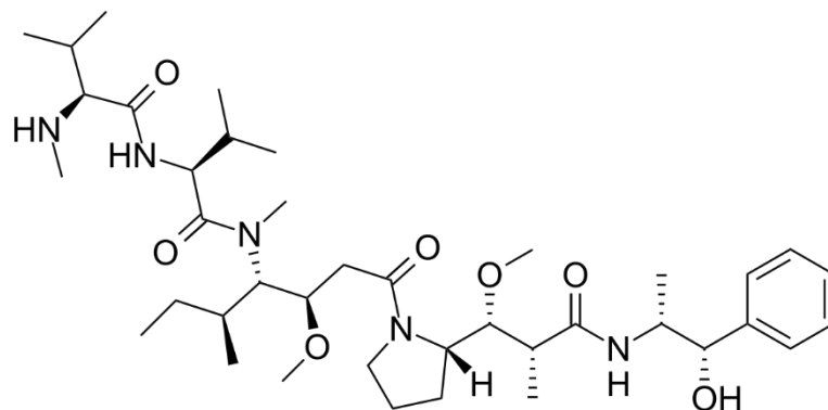
auristatin
